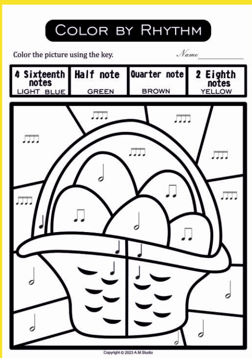
Set 2 Term-Symbol
