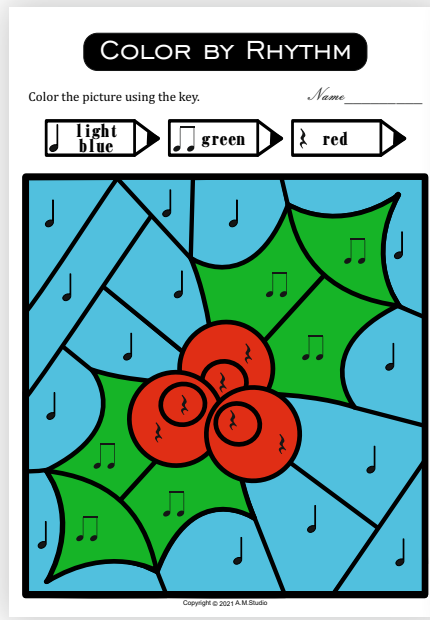
Set 2 Term-Symbol
